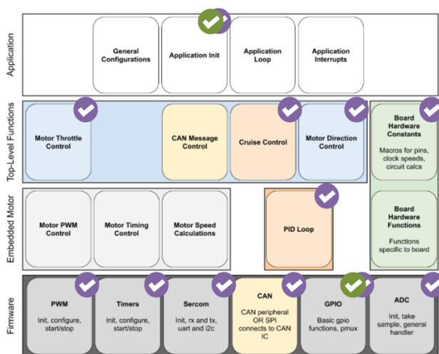
Figure 4. Software module implementation
