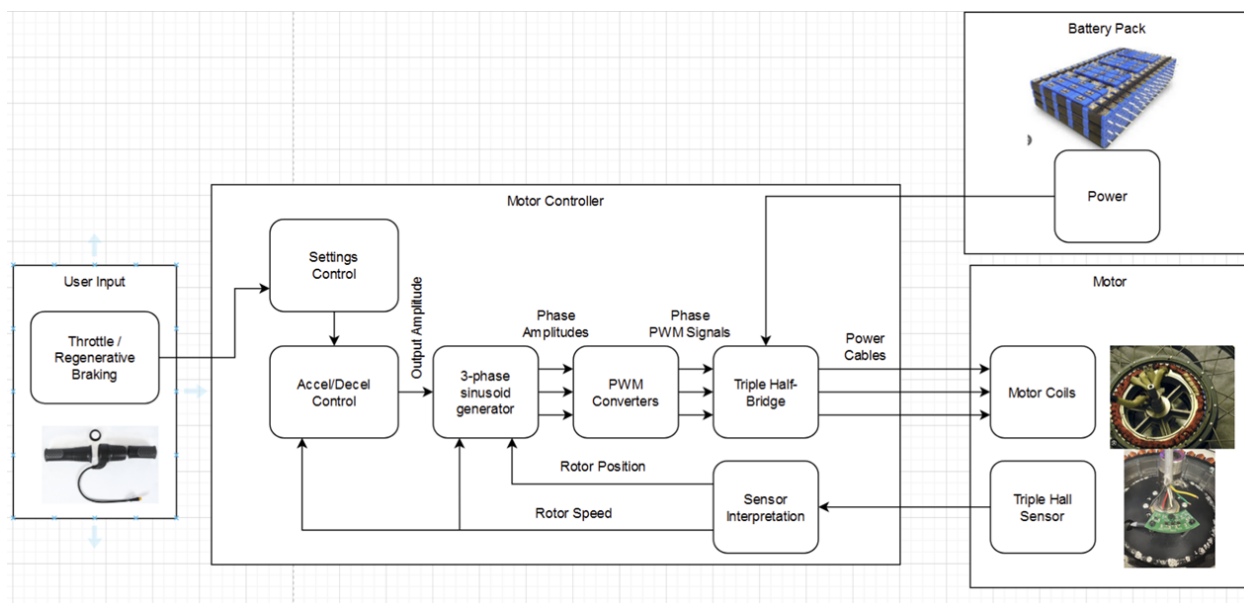
Figure 3. System design diagram
